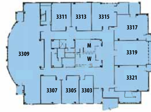
WEEKLEY BUILDING THIRD FLOOR
